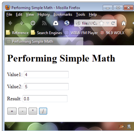
Figure 4-1: The example provides inputs and buttons for performing simple math tasks.
