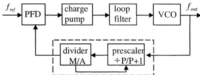
Figure 3-1. Charge-pump PLL frequency synthesizer
