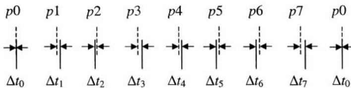
Figure 5-17. Phase mismatch in the phase-switching prescaler
