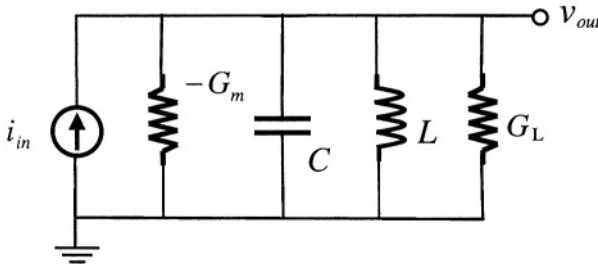
Figure 7-6. Simple LC oscillator noise model
