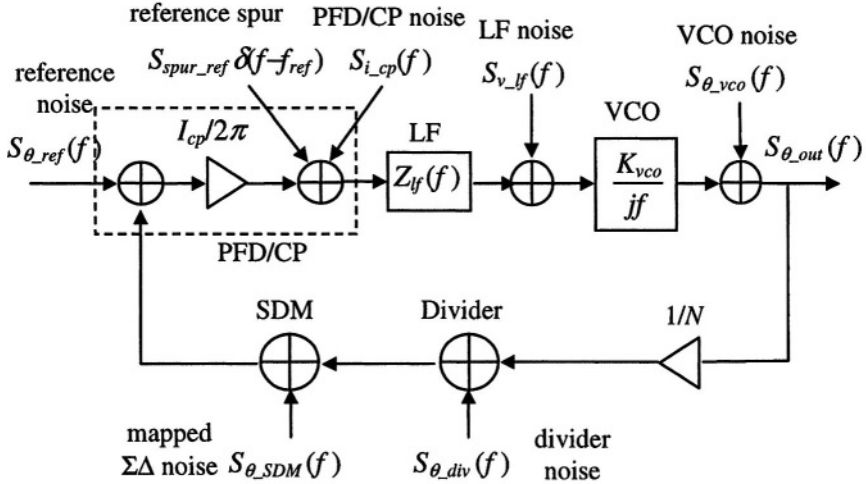
Figure 4-26. Frequency domain model of \Sigma\Delta -PLL
