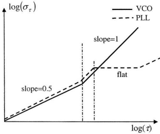
Figure 2-4. Timing jitter of VCO and PLL
