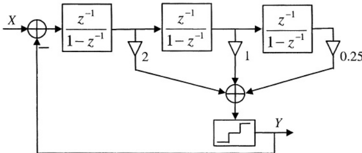
Figure 4-10. Single-stage multiple feedforward topology (FF3)
