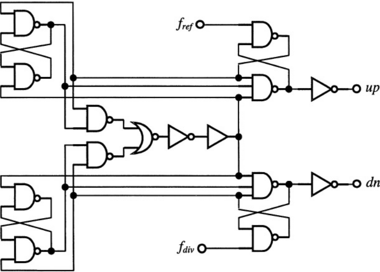
Figure 7-10. PFD using RS latch
