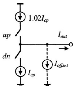
Figure 4-18. Charge-pump with current mismatch
