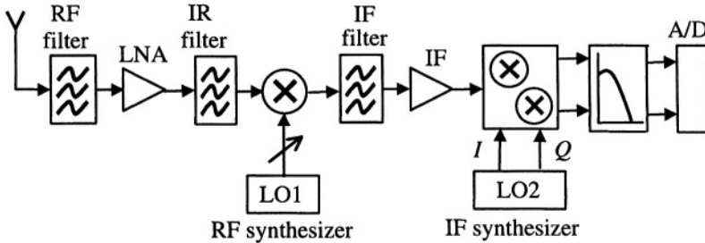
Figure 2-13. Super-heterodyne receiver architecture
