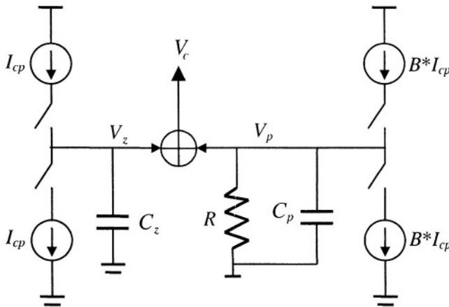
Figure 6-3. Dual-path loop filter
