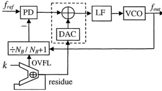
Figure 2-8. FN-FS using DAC phase interpolation
