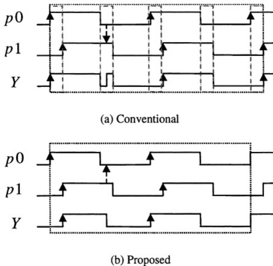
Figure 5-8. Phase-switching sequence
