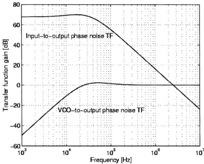
Figure 3-20. Bluetooth PLL closed-loop phase transfer function
