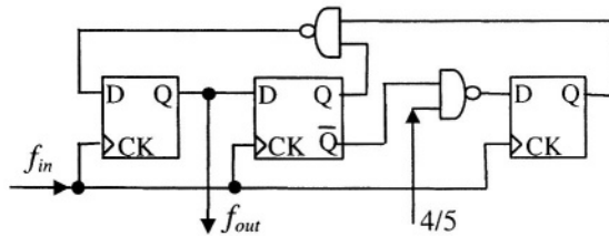
(a) Divide-by-4/5
