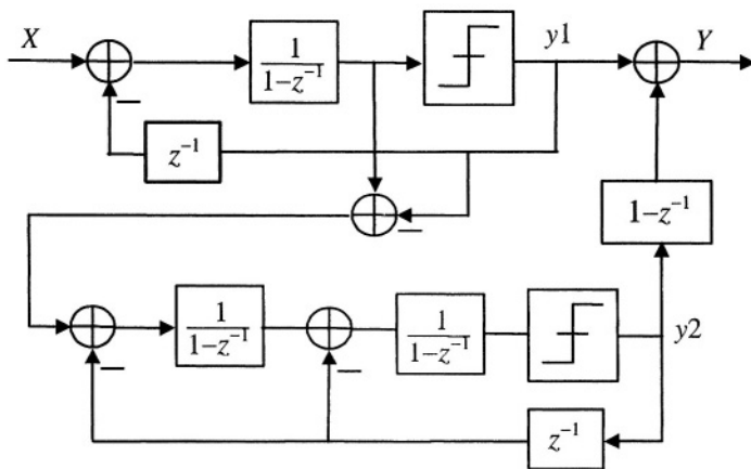
Figure 4-6. MASH 1-2 topology
