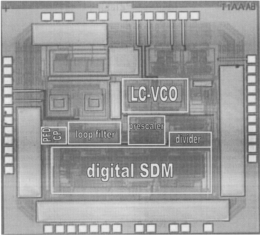
Figure 8-10. Microphotograph of the whole chip
