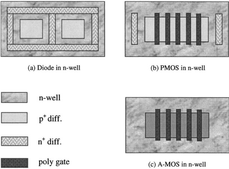
Figure 7-3. Top view of varactors in CMOS technology
