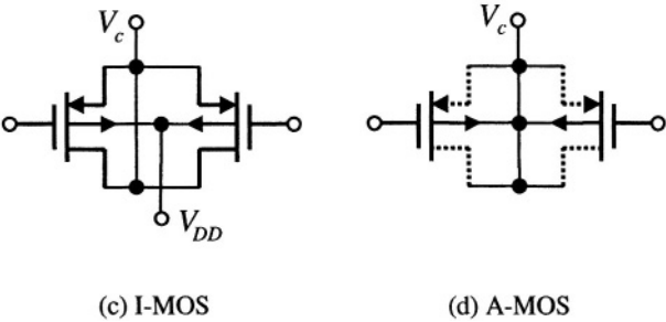
(c) I-MOS (d) A-MOS Figure 7-2. Different types of varactors (continued)
