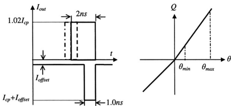
(a) Output current pulses
