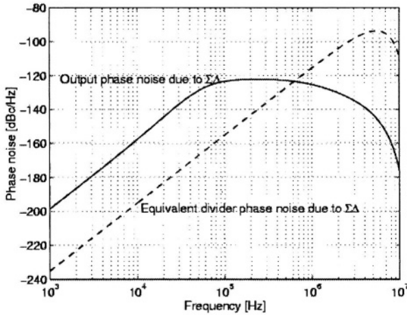
Figure 4-29. GSM PLL input-referred SD phase noise
