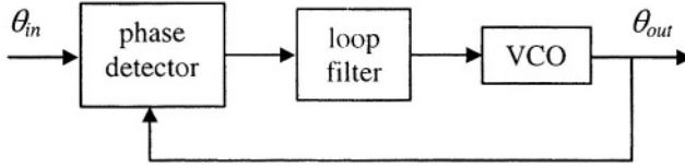
Figure 2-16. Basic PLL diagram
