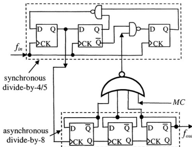
Figure 5-2. Conventional divide-by-32/33 prescaler
