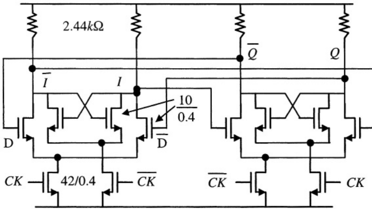
Figure 5-9. SCL flip-flop configured as divide-by-2
