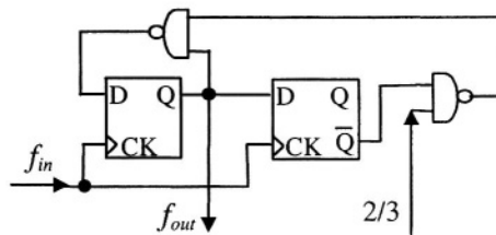
(c) Divide-by-2/3
