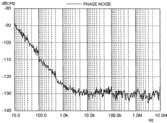
Figure 8-5. Measured residual phase noise
