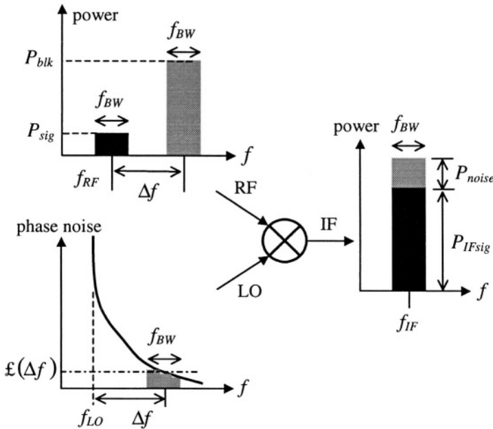
Figure 2-15. Down-conversion with phase noise
