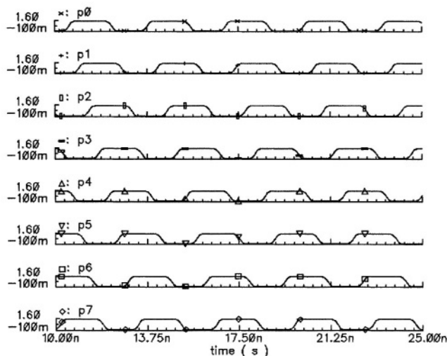
Figure 5-10. Simulated eight 45°-spaced divide-by-8 waveforms
