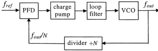
Figure 2-7. Integer-N PLL-FS
