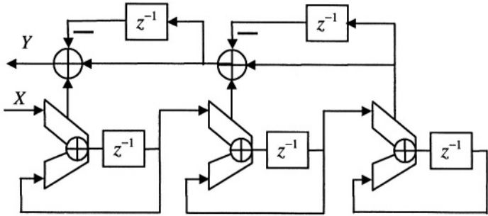
Figure 4-2. MASH 1-1-1 topology
