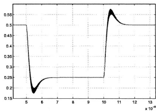
(c) \phi_m=53^\circ ( b=9 )
