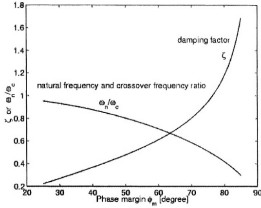
Figure 3-8. Natural frequency and damping factor vs. phase margin
