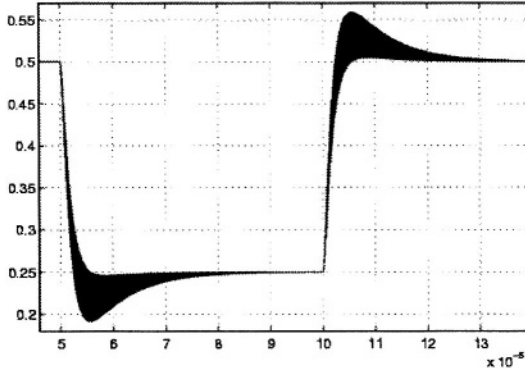
(e) \phi_m=71^\circ ( b=36 )
