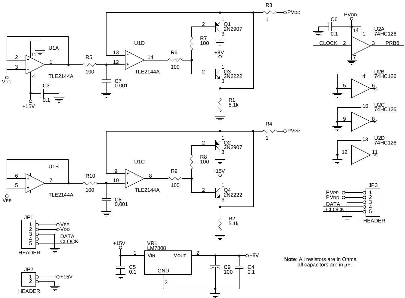
Figure 30-2: Example Driver Board Schematic
