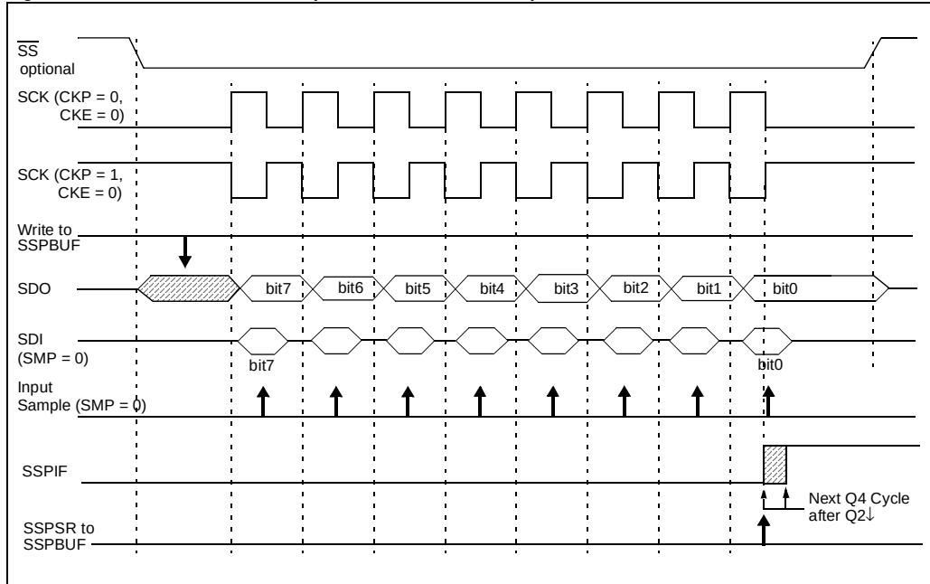
Figure 19-4: SPI Mode Waveform (Slave Mode With CKE = 0)
