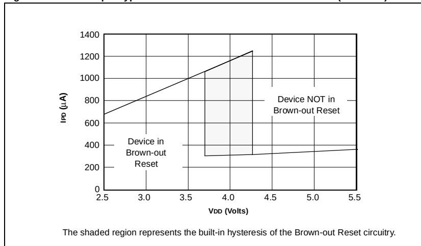
Figure 33-5: Example Typical I_{PD} vs. V_{DD} Brown-out Detect Enabled (RC Mode)
