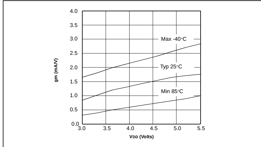
Figure 33-26: Example Transconductance (gm) of LP Oscillator vs. VDD
