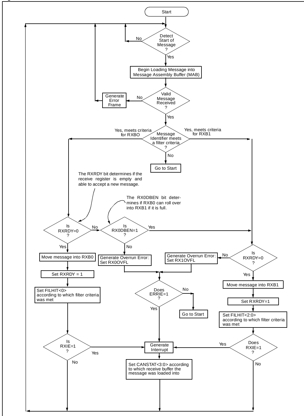
Figure 22-15:Receive Flowchart
