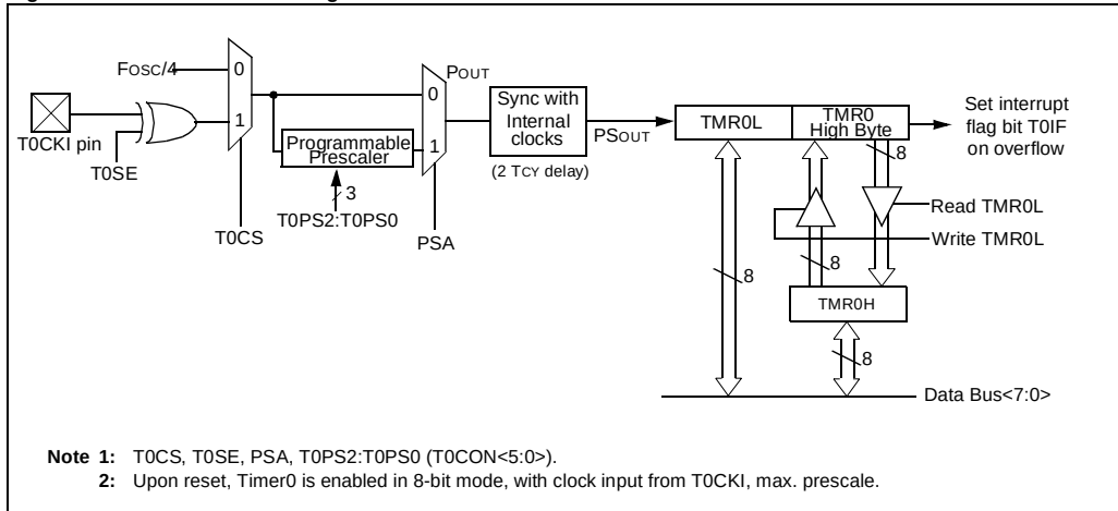
Figure 13-2: Timer0 Block Diagram in 16-bit Mode
