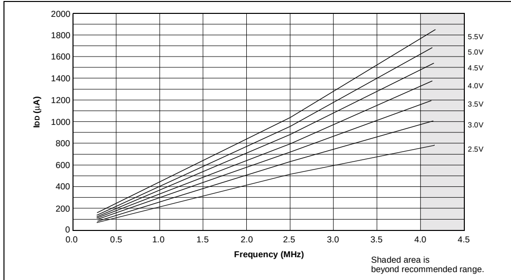
Figure 33-11: Example Typical I_{DD} vs. Frequency (RC Mode @ 100 pF, 25°C)
