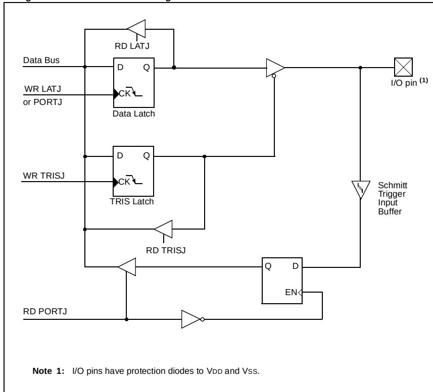
Figure 11-13: PORTJ Block Diagram
