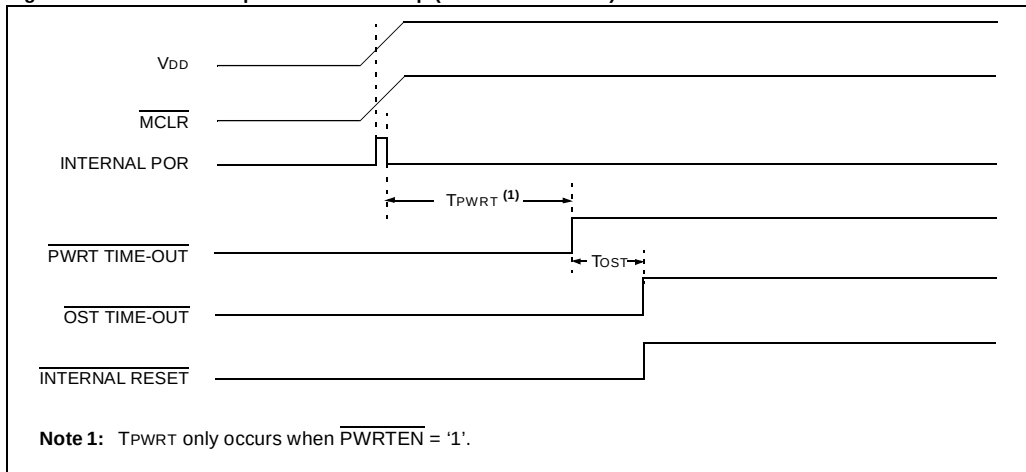
Figure 3-5: Time-out Sequence on Power-up ( \overline{\text{MCLR}} Tied to VDD)
