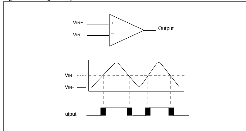
Figure 24-2: Single Comparator
