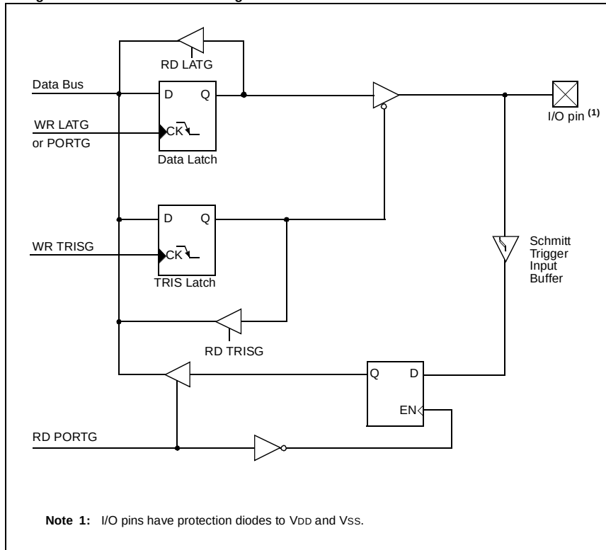
Figure 11-11: PORTG Block Diagram
