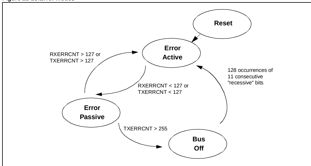
Figure 22-25: Error Modes
