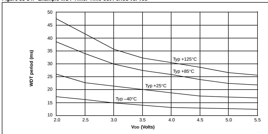
Figure 33-34: Example WDT Timer Time-out Period vs. V_{DD}
