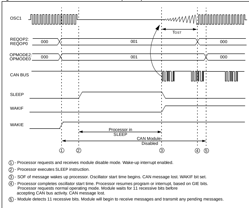
Figure 22-13: Processor SLEEP and CAN Bus Wake-up Interrupt
