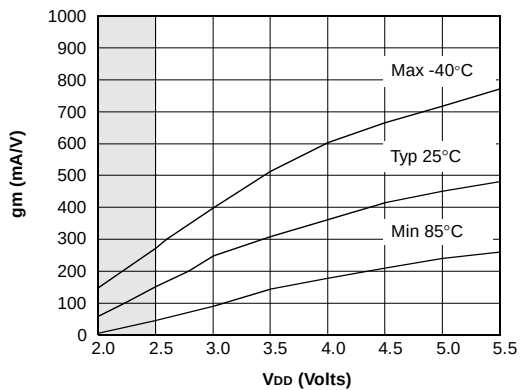
Figure 33-27: Example Transconductance (gm) of XT Oscillator vs. V DD
