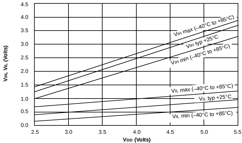
Figure 33-32: Example V_{IH} , V_{IL} of MCLR, T0CKI and OSC1 (in RC Mode) vs. V_{DD}
