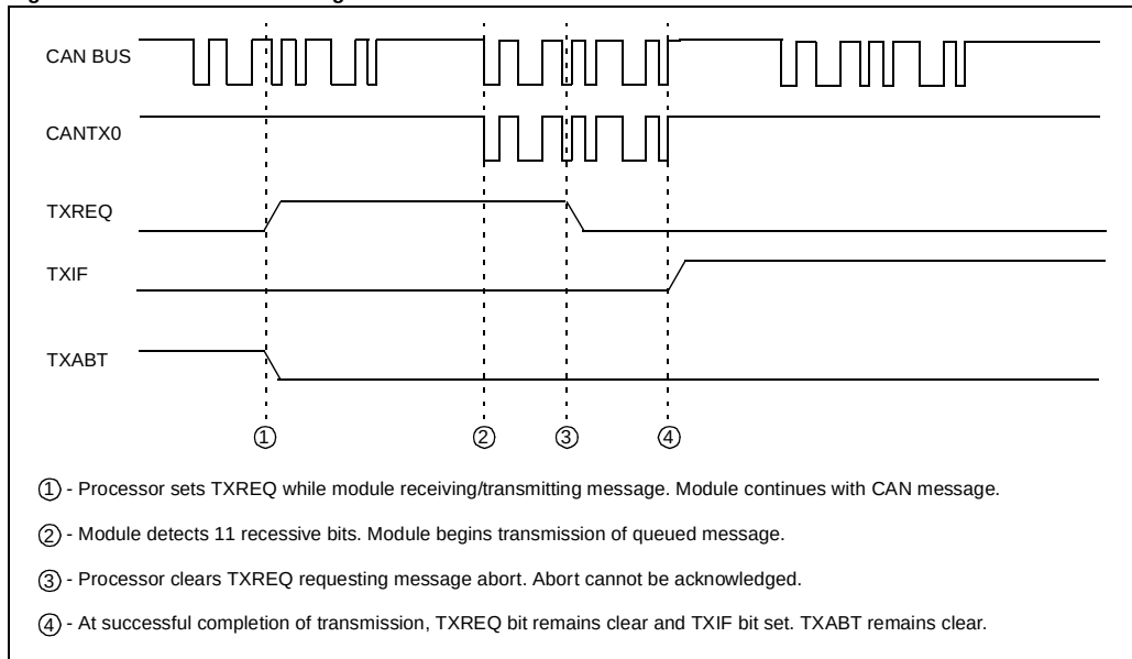
Figure 22-22: Failed Abort During Transmission
