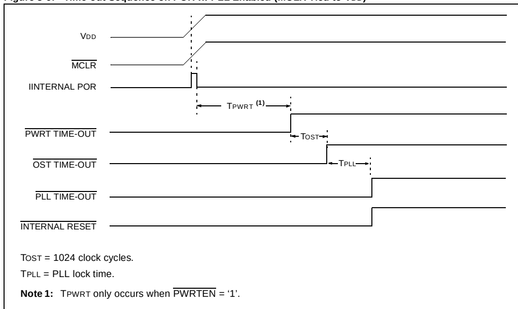
Figure 3-9: Time-out Sequence on POR w/ PLL Enabled (MCLR Tied to V DD )
