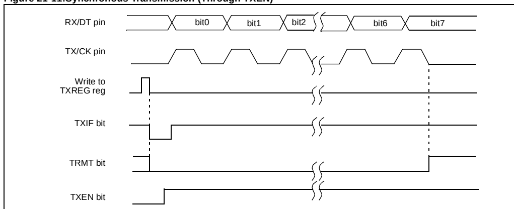
Figure 21-11: Synchronous Transmission (Through TXEN)
