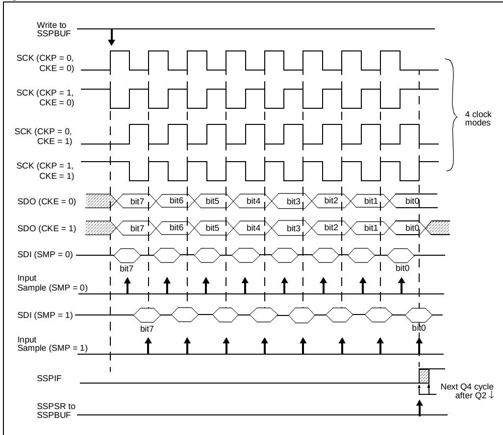
Figure 19-3: SPI Mode Waveform, Master Mode
