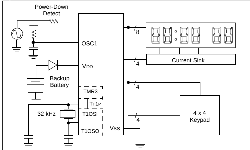
Figure 16-4: Timer3 Application
