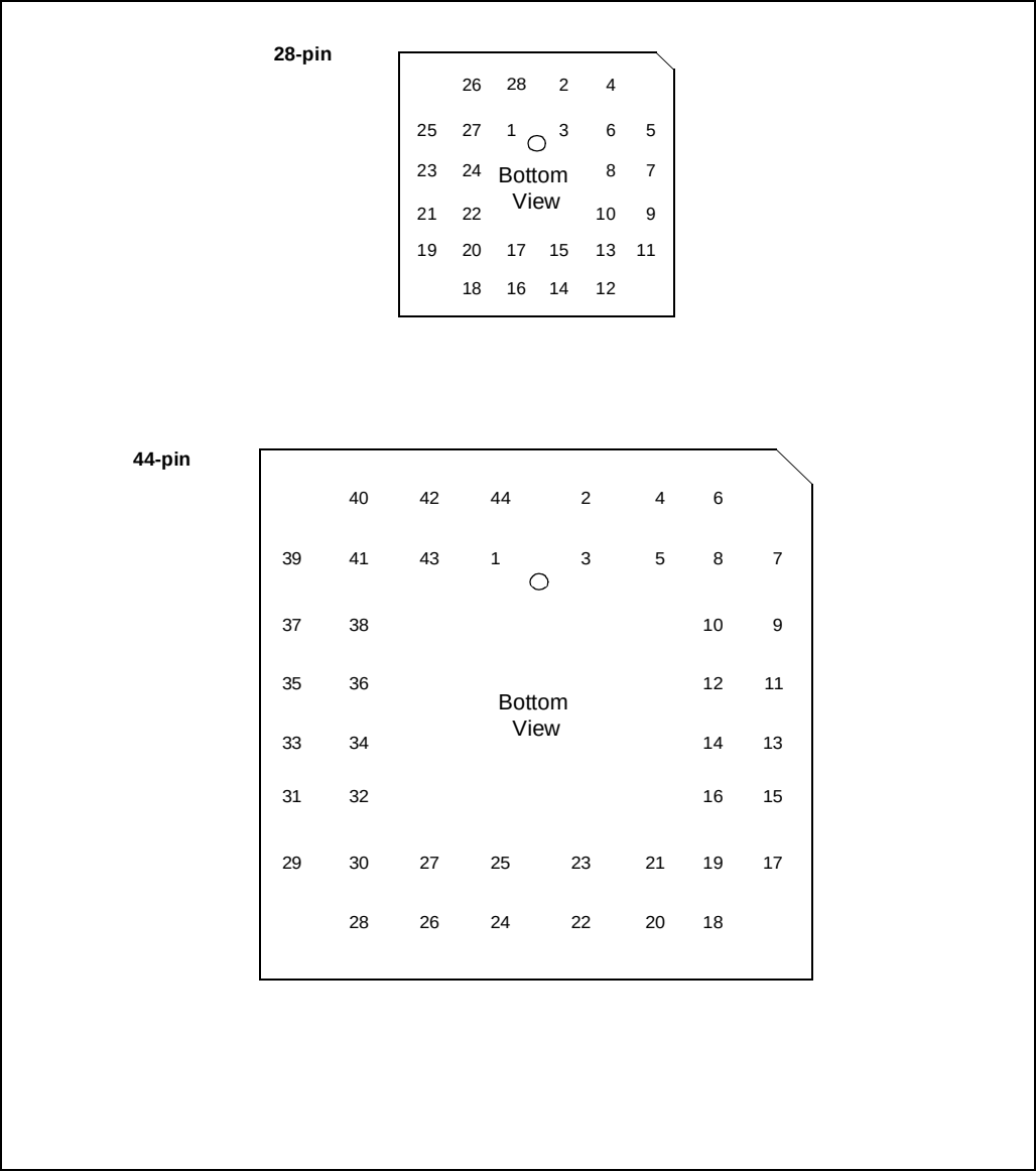
Figure G-2: PGA Package Pinout (Bottom View) for LCC Packages
