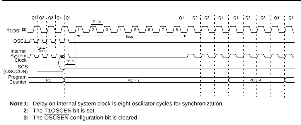
Figure 2-12: Transition From OSC1 to Timer1 Oscillator Waveform
