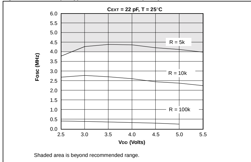
Figure 33-23: Example Typical RC Oscillator Frequency vs. VDD
