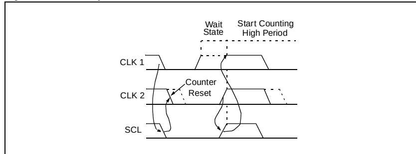
Figure A-10:Clock Synchronization
