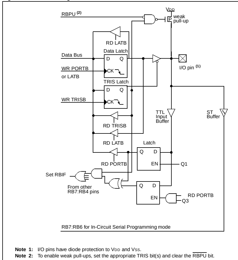
Figure 11-5: Block Diagram of RB7:RB4 Pins
