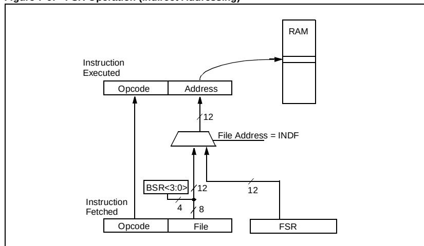
Figure 7-9: FSR Operation (Indirect Addressing)
