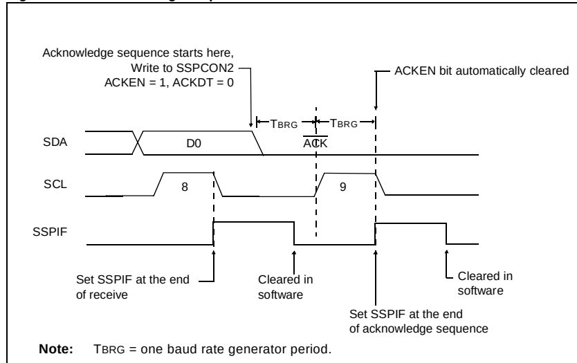
Figure 20-29: Acknowledge Sequence Waveform
