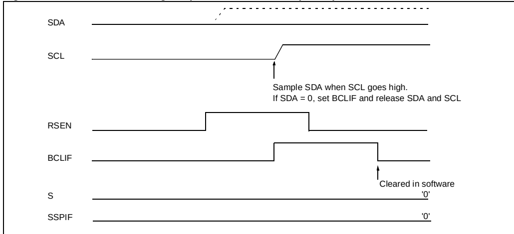
Figure 20-39: Bus Collision During Repeated Start Condition (Case 2)
