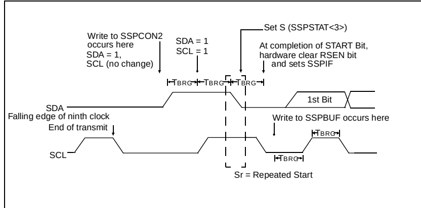
Figure 20-22: Repeat Start Condition Waveform
