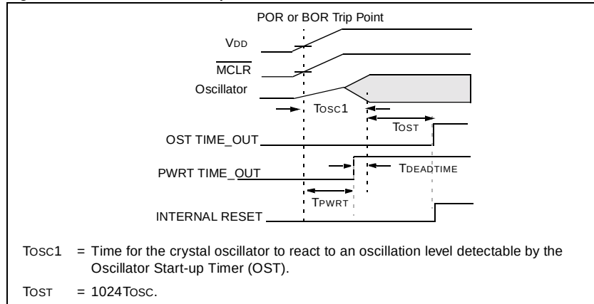
Figure 3-4: Oscillator Start-up Time
