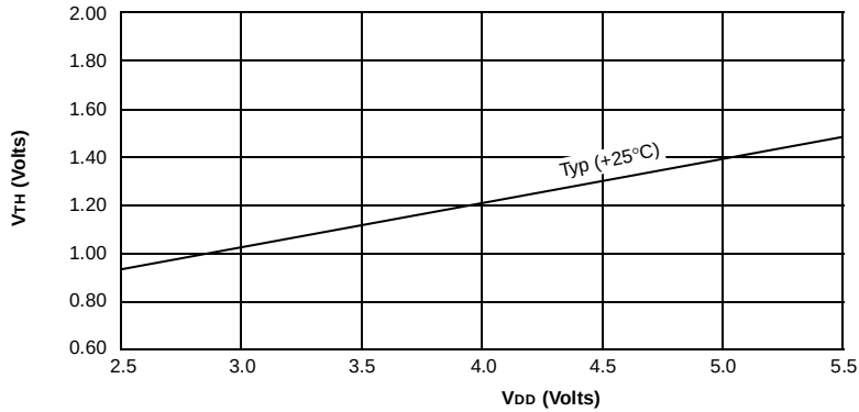
Figure 33-31: Example V_{TH} (Input Threshold Trip Point Voltage) of I/O Pins vs. V_{DD}
