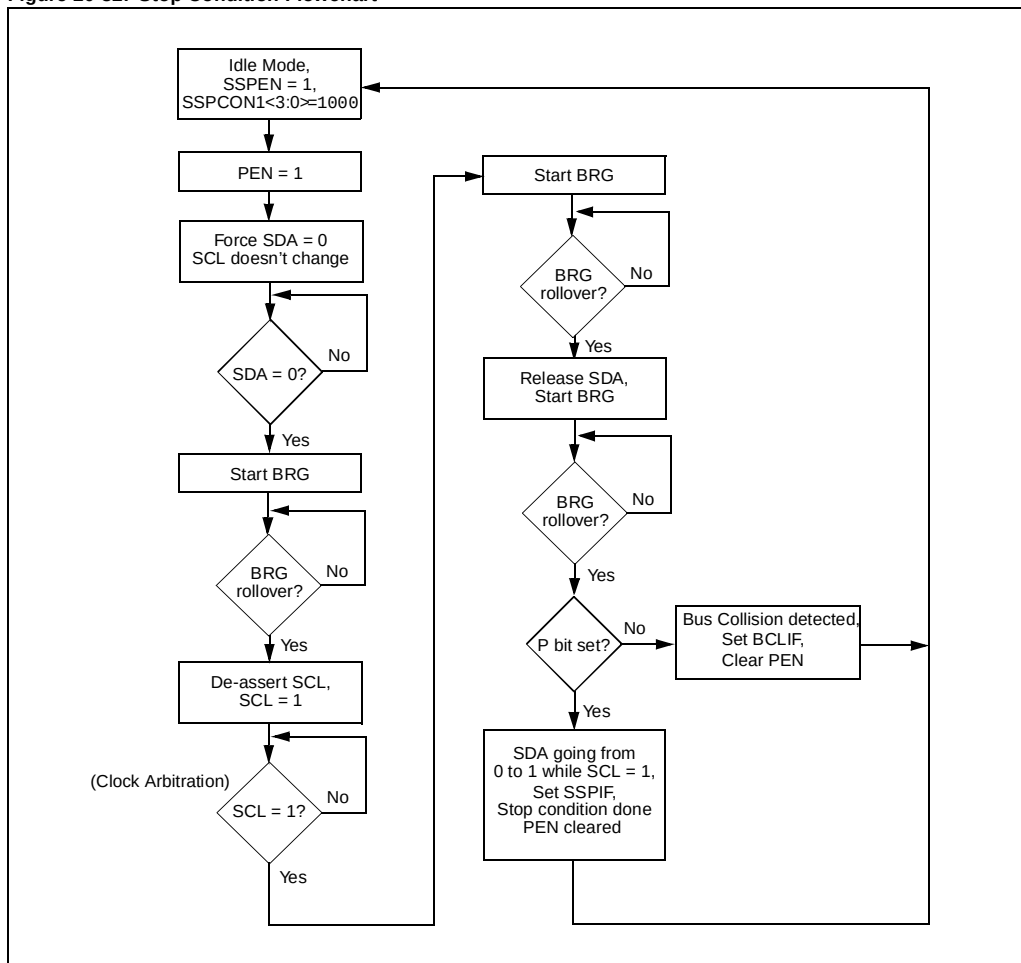
Figure 20-32: Stop Condition Flowchart
