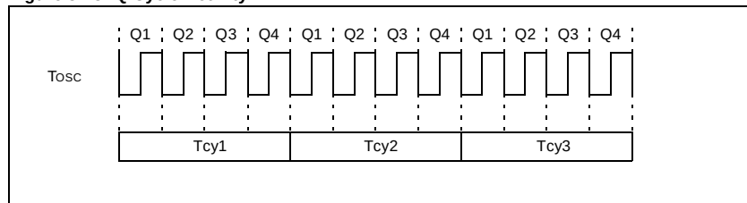
Figure 31-3: Q Cycle Activity
