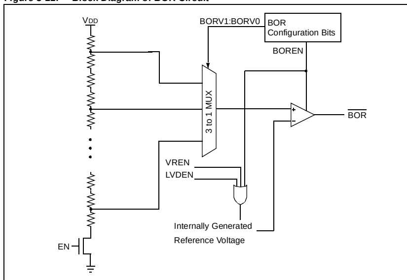
Figure 3-11: Block Diagram of BOR Circuit
