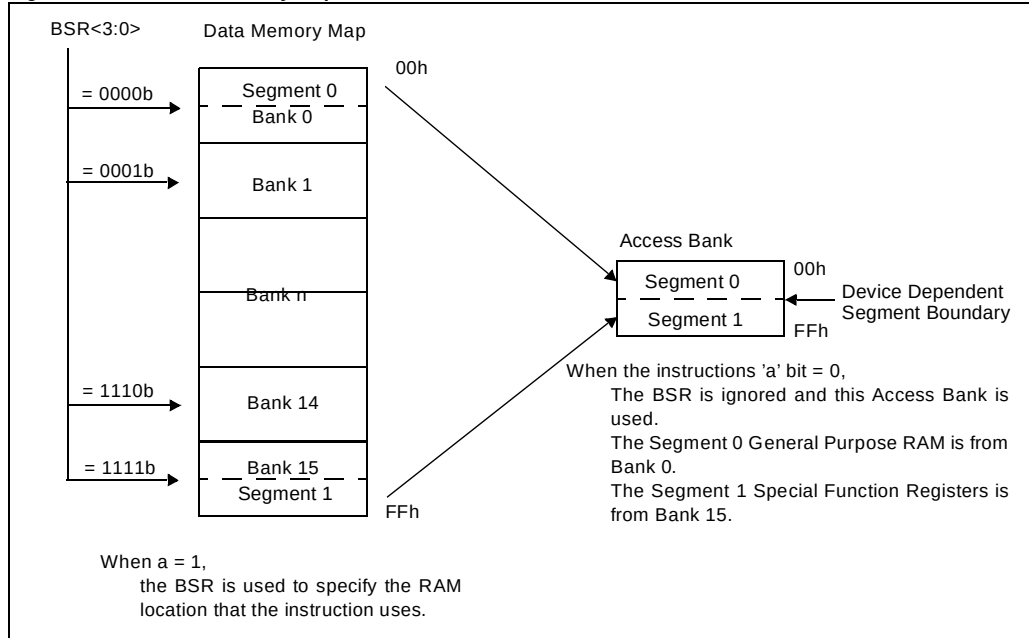
Figure 31-1: The Data Memory Map and the Access Bank
