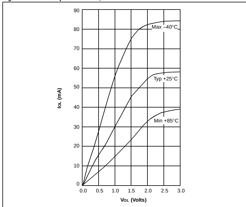
Figure 33-38: Example I_{OL} vs. V_{OL} , V_{DD} = 5\text{ V}
