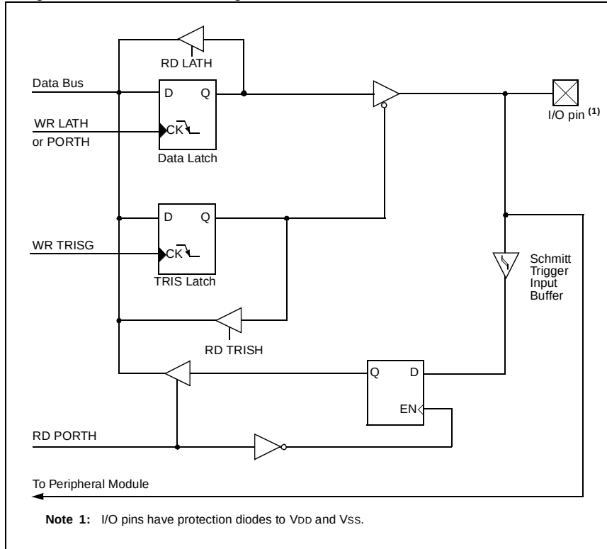
Figure 11-12: PORTH Block Diagram
