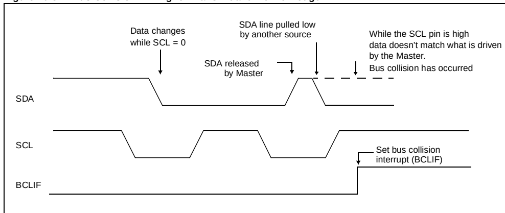
Figure 20-34: Bus Collision Timing for Transmit and Acknowledge
