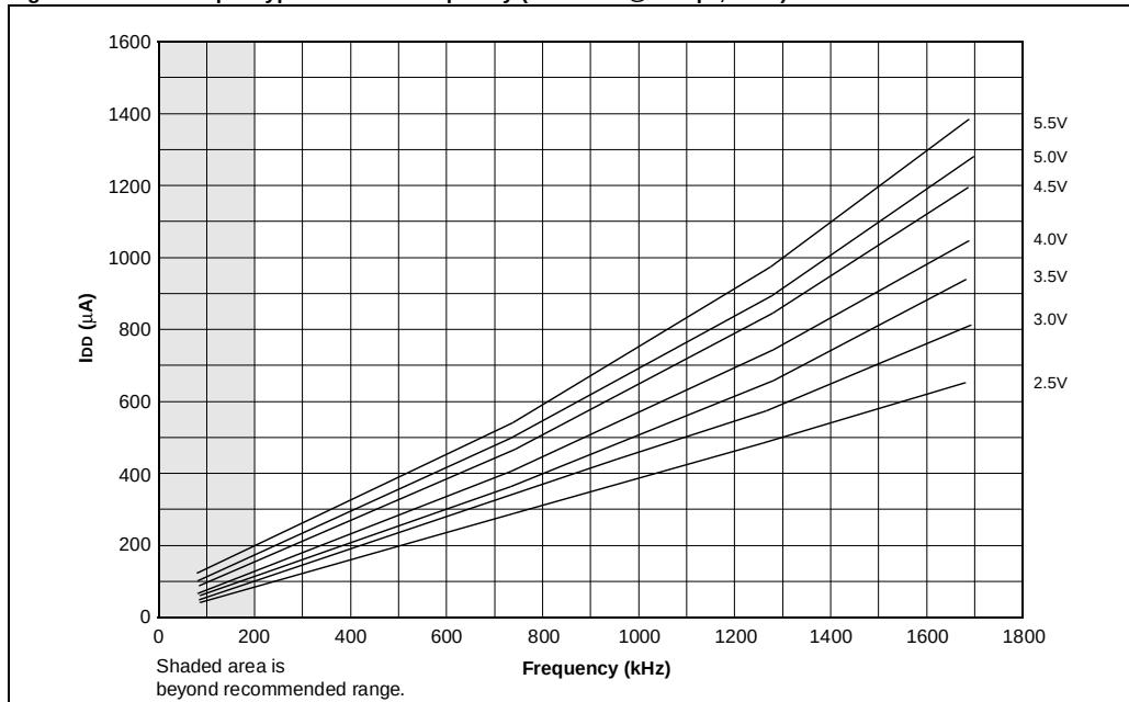
Figure 33-11: Example Typical I_{DD} vs. Frequency (RC Mode @ 100 pF, 25°C)
