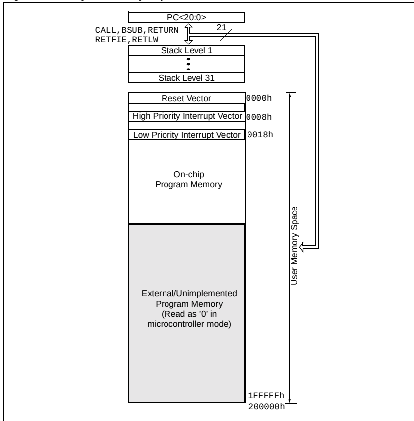
Figure 7-1: Program Memory Map and Stack for PIC18CXX
