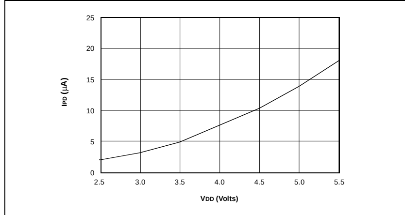
Figure 33-4: Example Maximum I_{PD} vs. V_{DD} (WDT Enabled, RC Mode)
