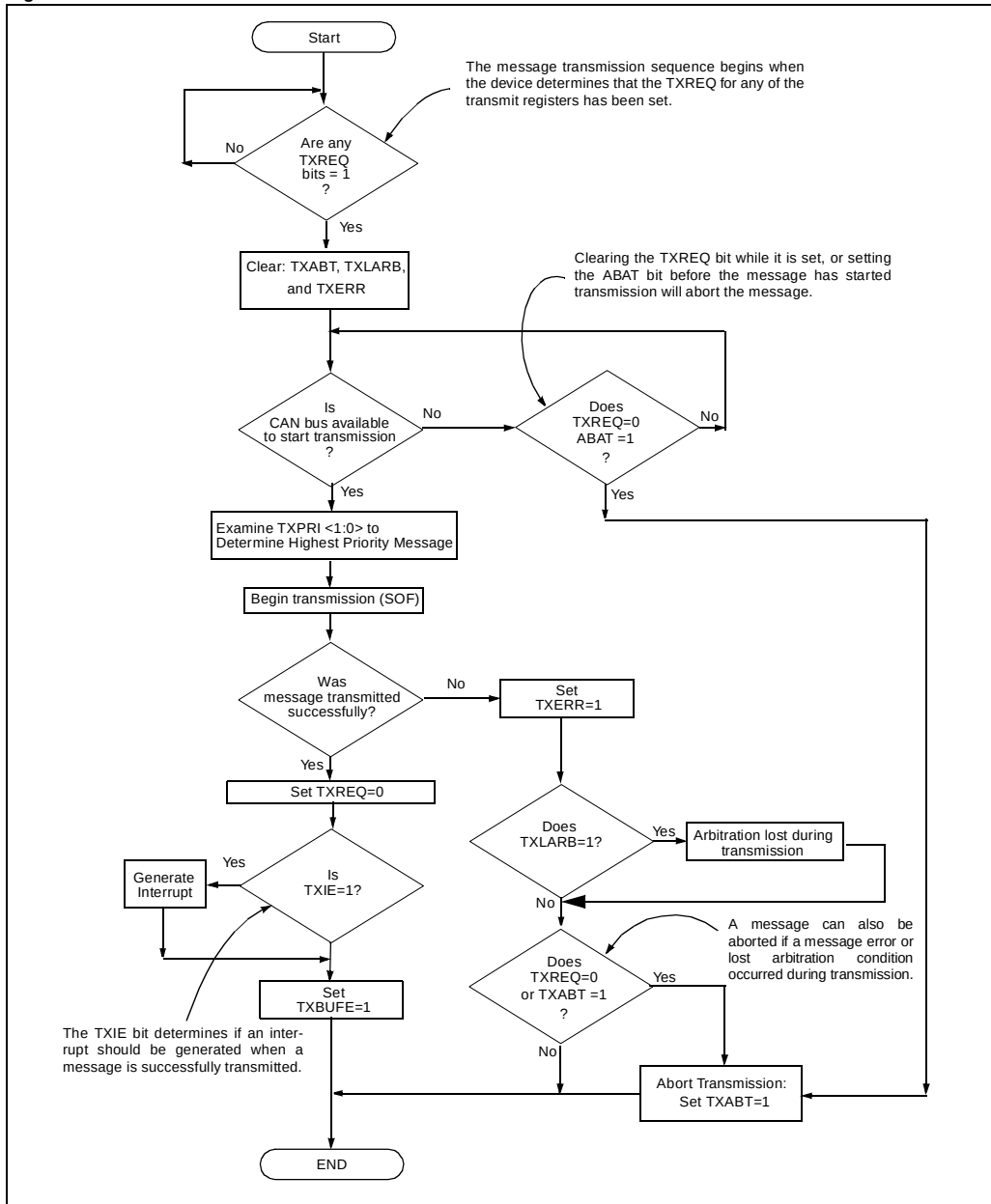
Figure 22-19: Transmit Flowchart
