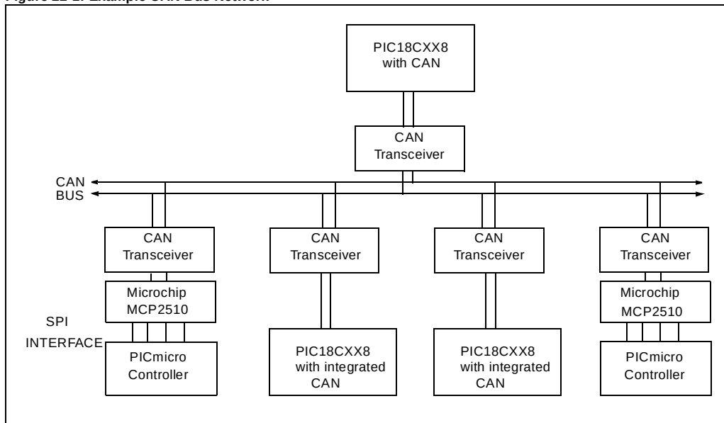
Figure 22-1: Example CAN Bus Network
