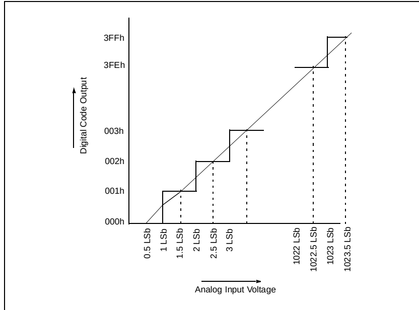
Figure 26-7: A/D Transfer Function
