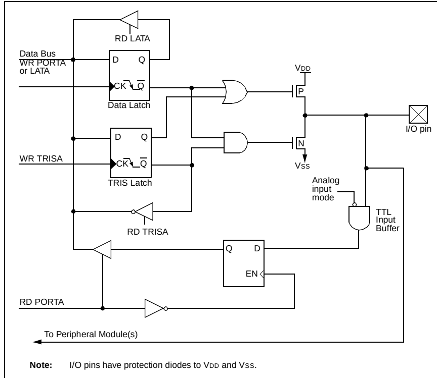
Figure 11-2: Block Diagram of RA3:RA0 and RA5 Pins
