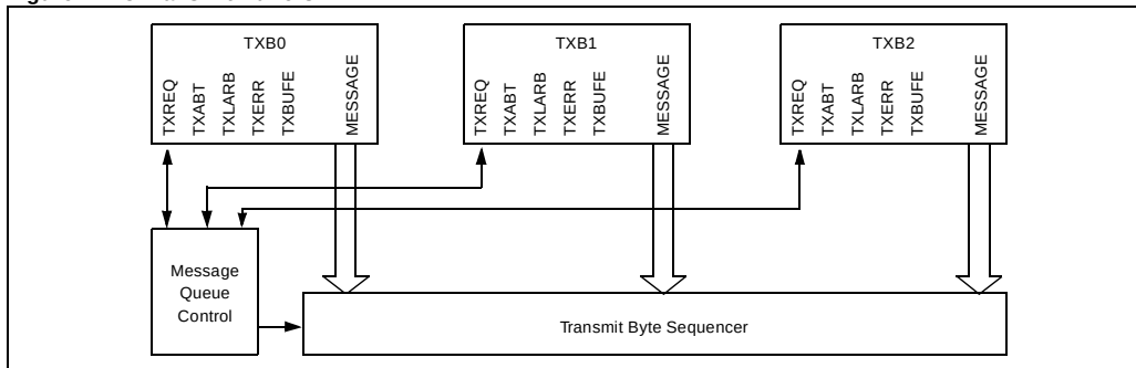
Figure 22-18: Transmit Buffers
