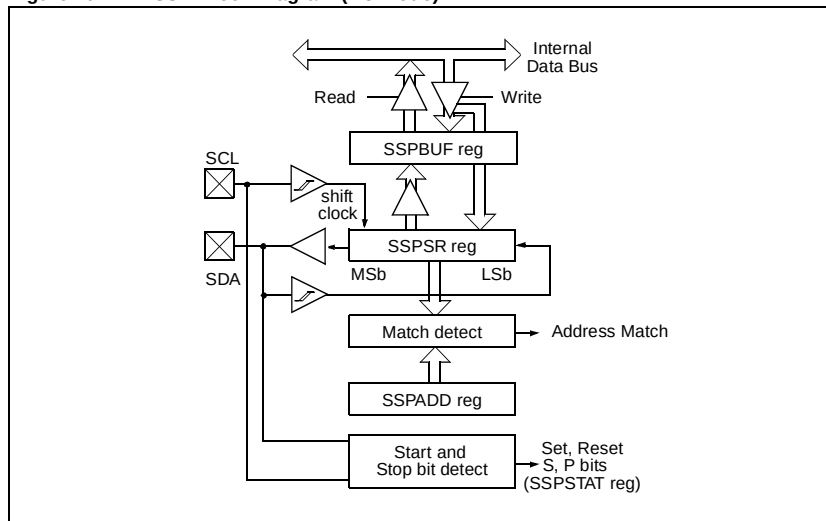
Figure 19-7: SSP Block Diagram (I 2 C Mode)
