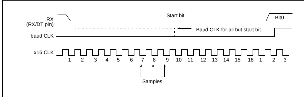
Figure 21-9: RX Pin Sampling Scheme, BRGH = 0 or BRGH = 1
